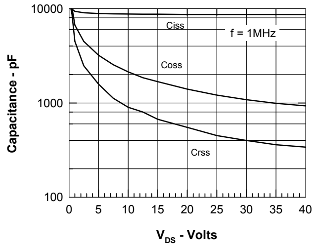
Figure 8. Capacitance Curves
