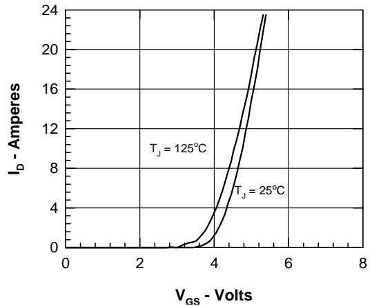
Figure 6. Admittance Curves
