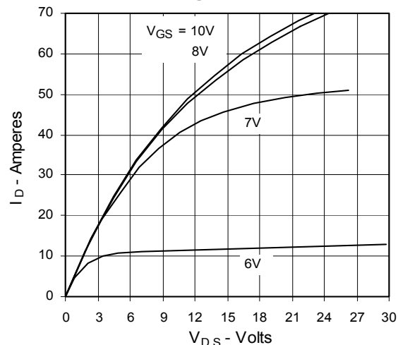
Fig. 2. Extended Output Characteristics @ 25^\circ\text{C}
