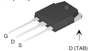
TO-3P (IXTQ)
