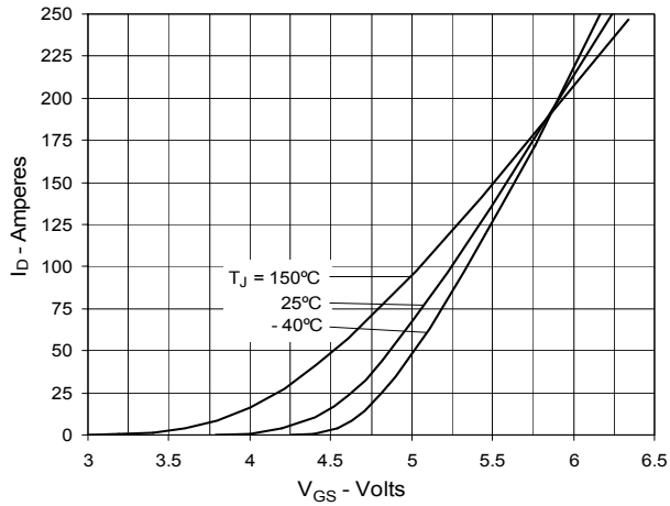
Fig. 7. Input Admittance
