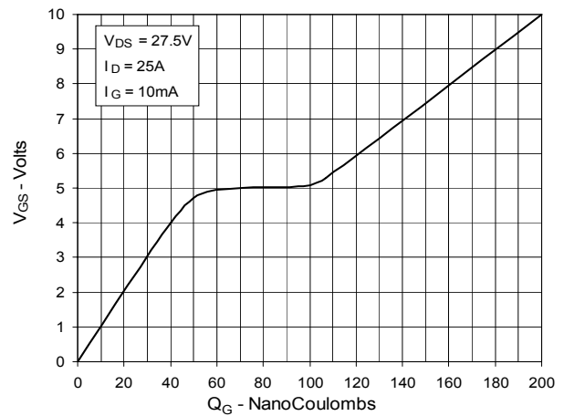
Fig. 10. Gate Charge
