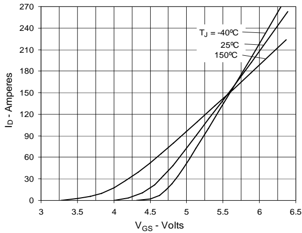
Fig. 7. Input Admittance
