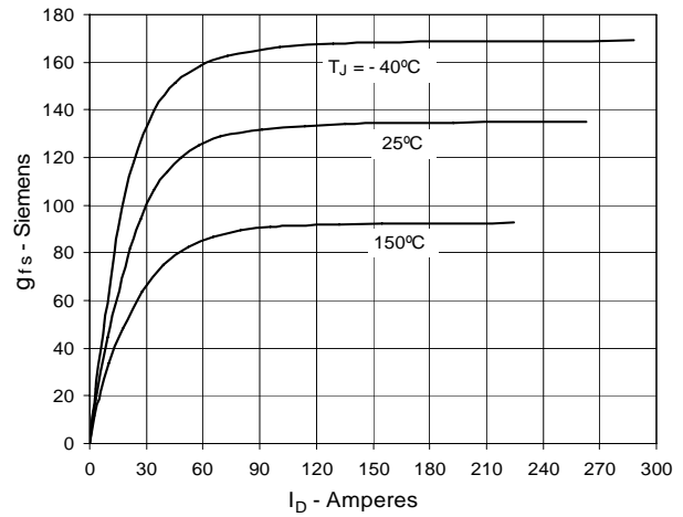
Fig. 8. Transconductance
