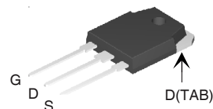
TO-3P (IXTQ)
