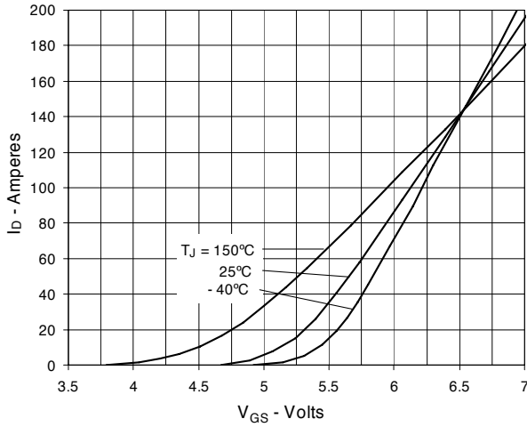
Fig. 7. Input Admittance
