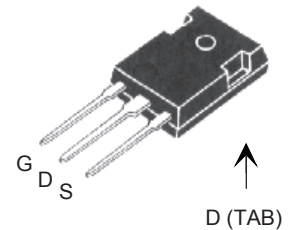
TO-247 (IXFH)
