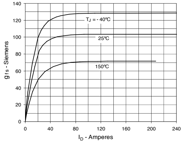
Fig. 8. Transconductance
