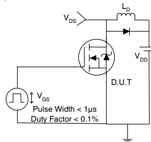
Fig 19a. Switching Time Test Circuit
