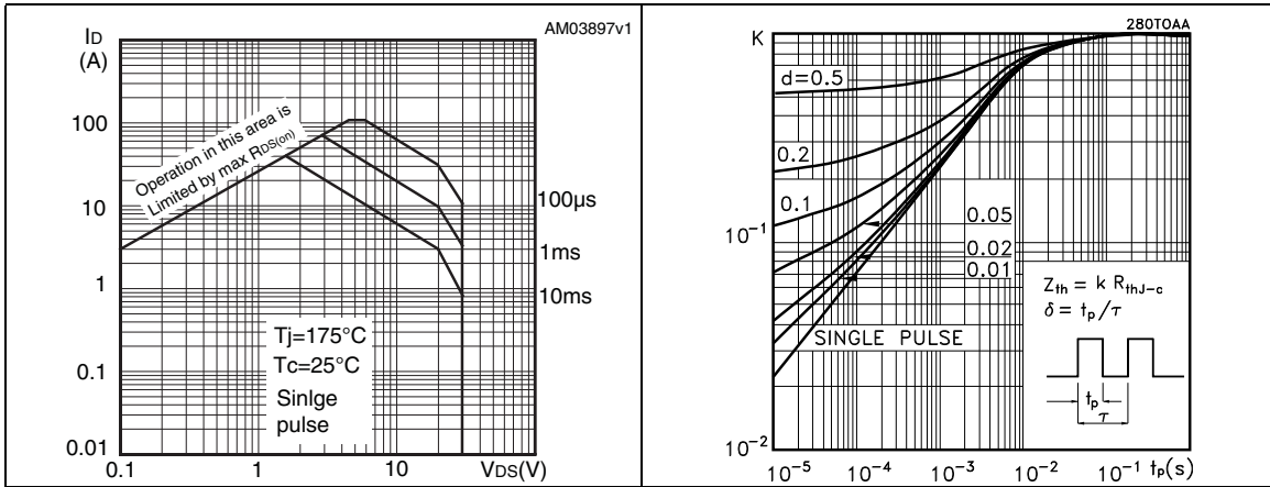
Figure 4. Safe operating area for DPAK, IPAK Figure 5. Thermal impedance for DPAK, IPAK
