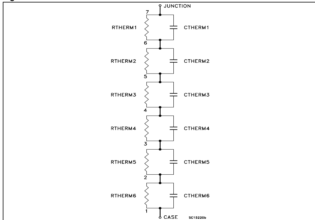
Figure 19. Thermal network
