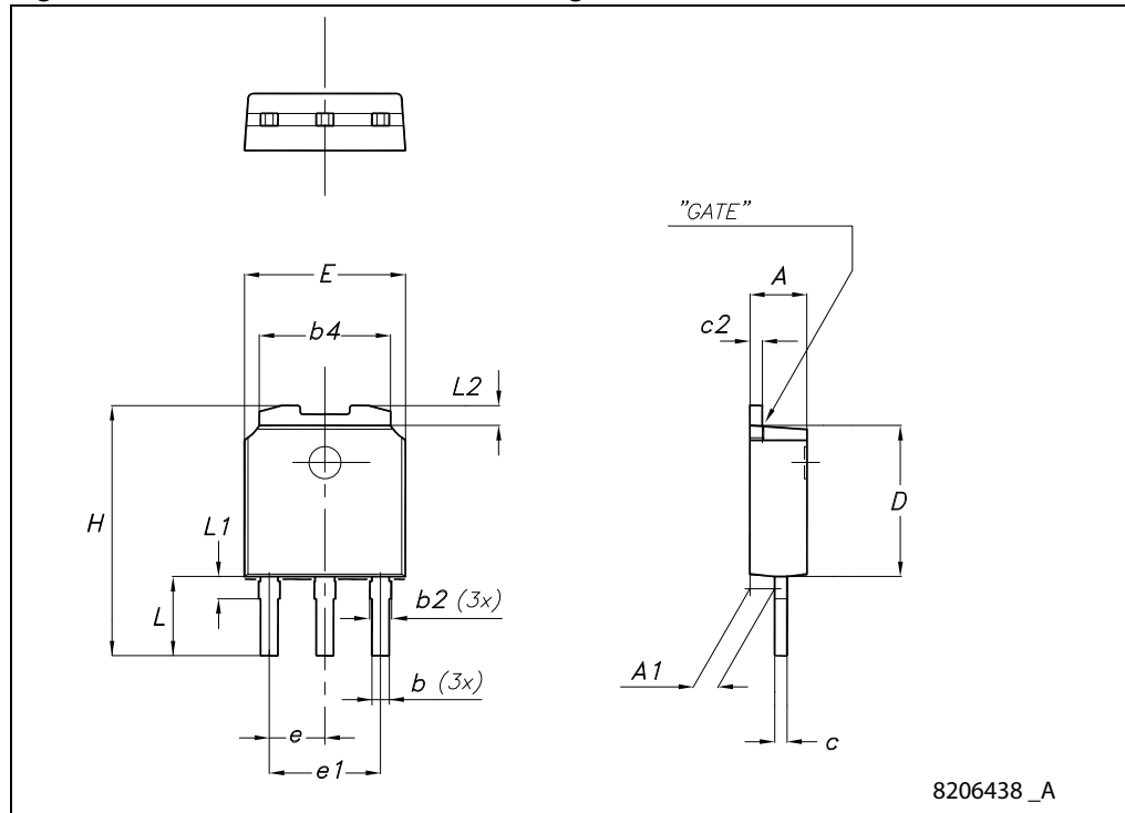
Figure 20. Short IPAК mechanical drawing
