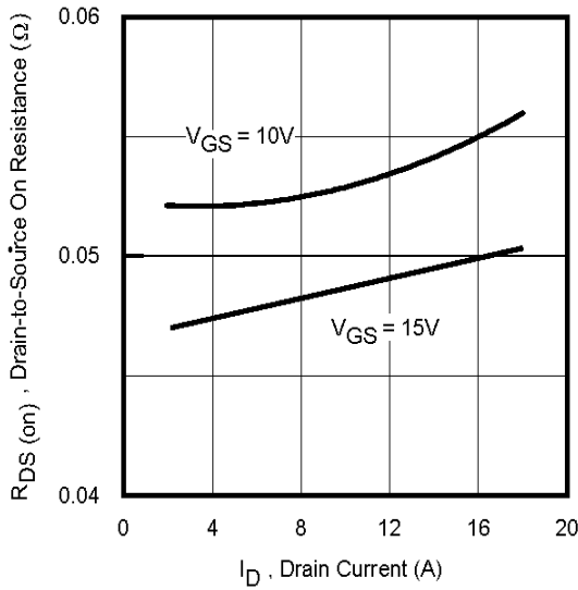
Fig 12. On-Resistance Vs. Drain Current
