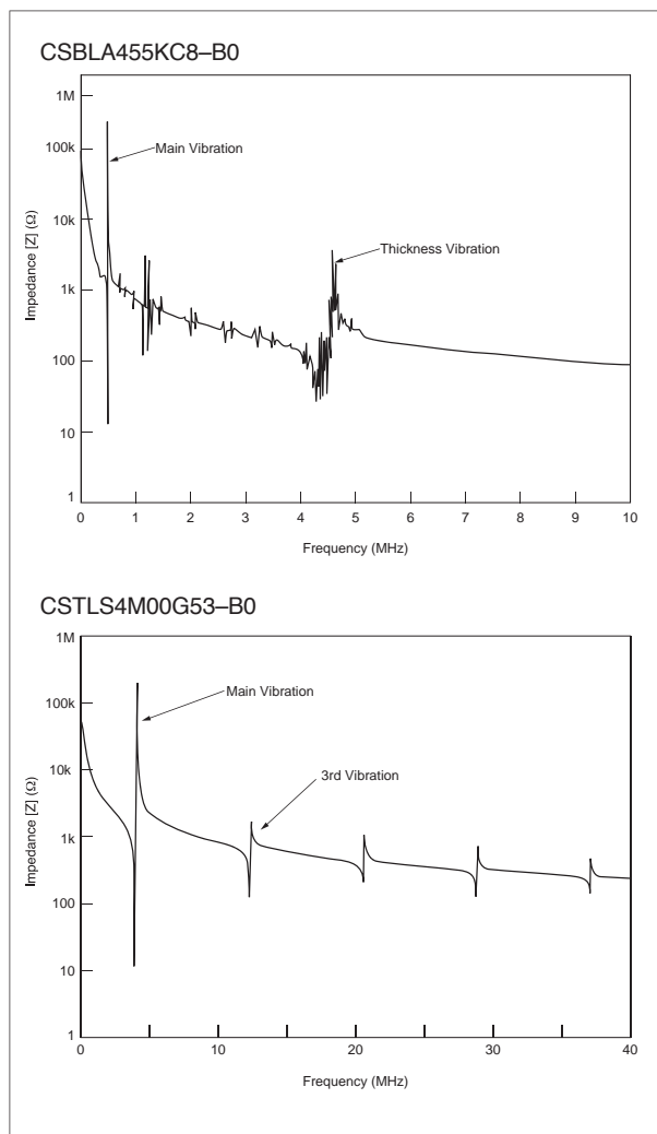
Fig. 2-5 Spurious Characteristics of CERALOCK®
