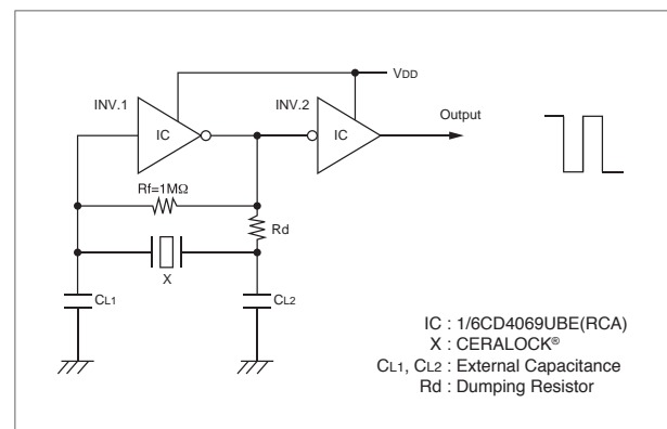
Fig. 4-1 Basic Oscillation Circuit with C-MOS Inverter
