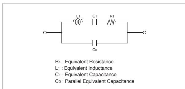
Fig. 2-3 Electrical Equivalent Circuit of CERALOCK®
