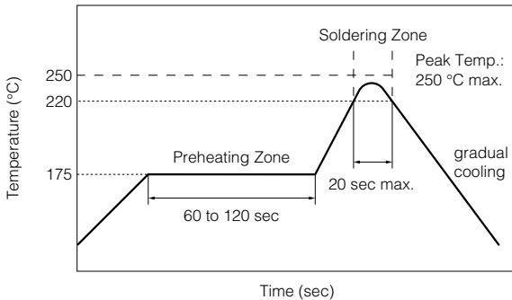
Fig. 1 Recommended Soldering Temperature-Time profile (Reflow Soldering)
