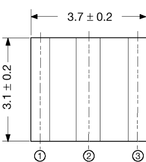
Figure 1) ECS-CR2-B Series - Top and Side Views
