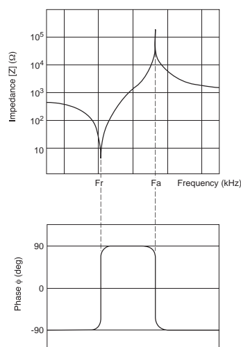
Fig. 2-2 Impedance and Phase Characteristics of CERALOCK®
