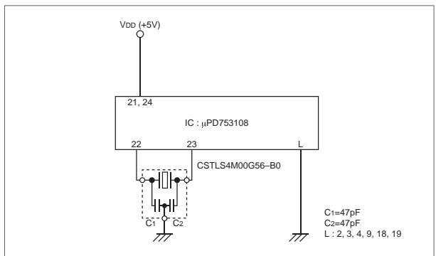
Fig. 6-4 Application to μPD753108 (Renesas Electronics)
