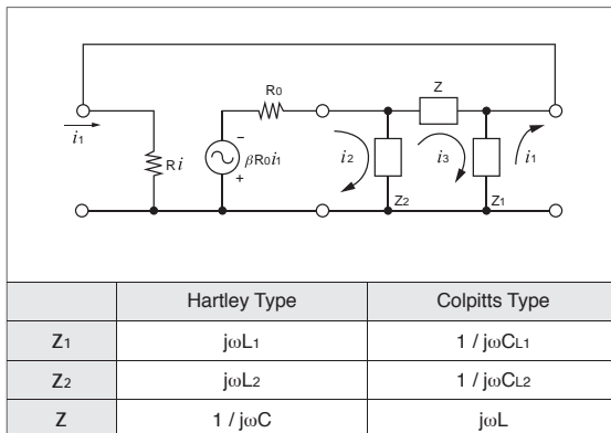
Fig. IV Hartley/Colpitts Type LC Oscillation Circuits
