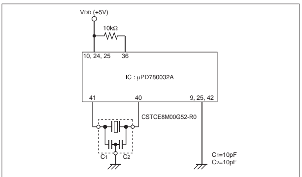
Fig. 6-7 Application to μPD780032A (Renesas Electronics)
