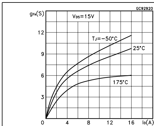
Figure 6. Transconductance
