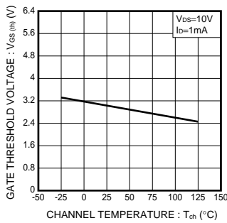
Fig.4 Gate Threshold Voltage vs. Channel Temperature
