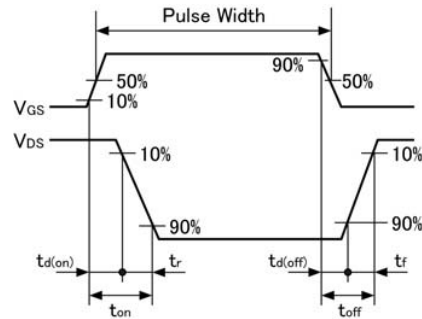
Fig.1-2 Switching waveforms
