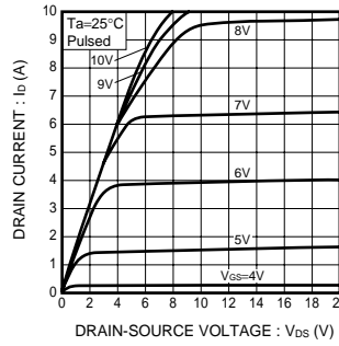
Fig.2 Typical Output Characteristics
