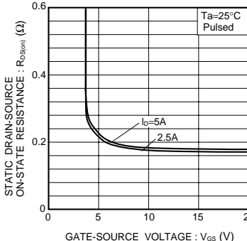
Fig.7 Static Drain-Source On-State Resistance vs. Gate-Source Voltage
