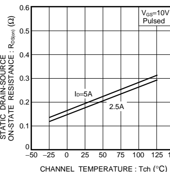
Fig.8 Static Drain-Source On-State Resistance vs. Channel Temperature
