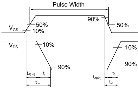
Fig.17 Switching Time Waveforms
