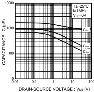
Fig.1 Typical Capacitance vs. Drain-Source Voltage
