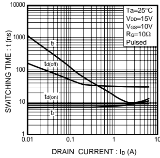
Fig.2 Switching Characteristics
