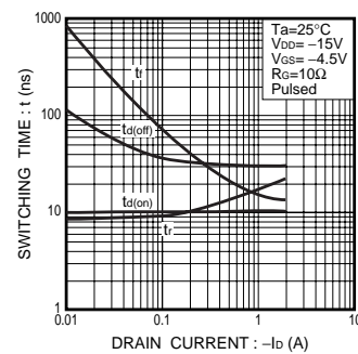
Fig.9 Switching Characteristics
