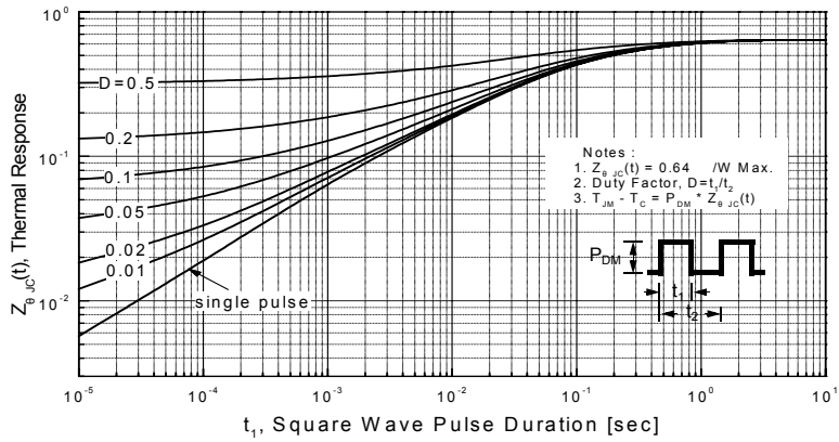
Figure 11-2. Transient Thermal Response Curve for FQPF13N50CF
