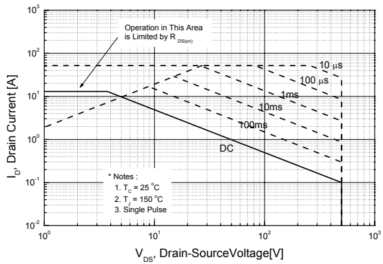
Figure 9-2. Maximum Safe Operating Area for FQPF13N50CF
