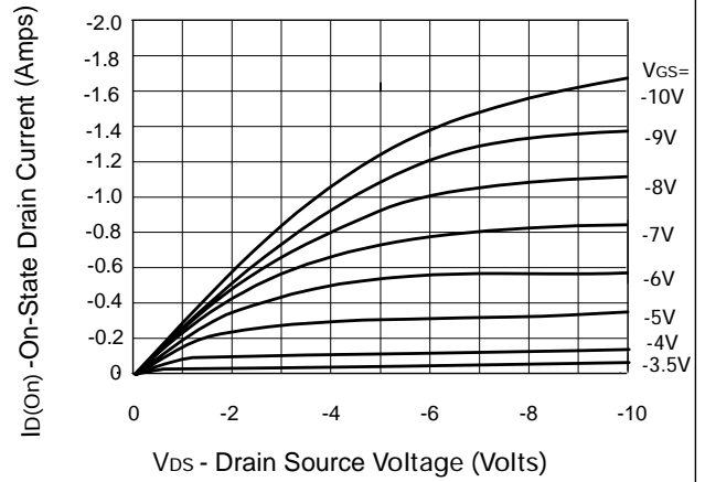
Saturation Characteristics
