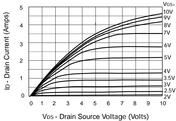
Saturation Characteristics
