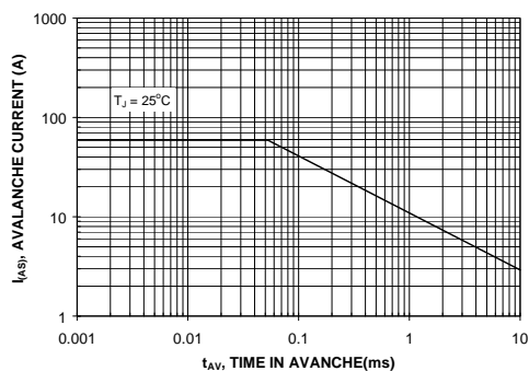
Figure 12. Unclamped Inductive Switching Capability
