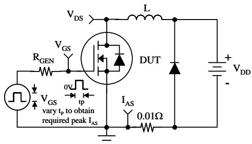
Figure 14. Unclamped Inductive Load Test Circuit
