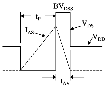
Figure 15. Unclamped Inductive Waveforms
