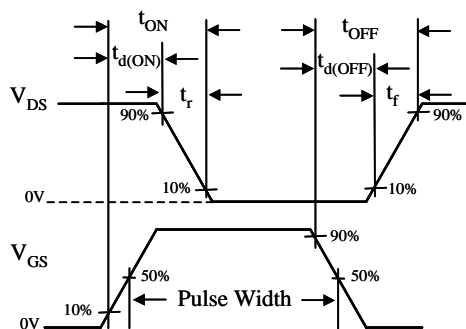
Figure 19. Switching Time Waveforms
