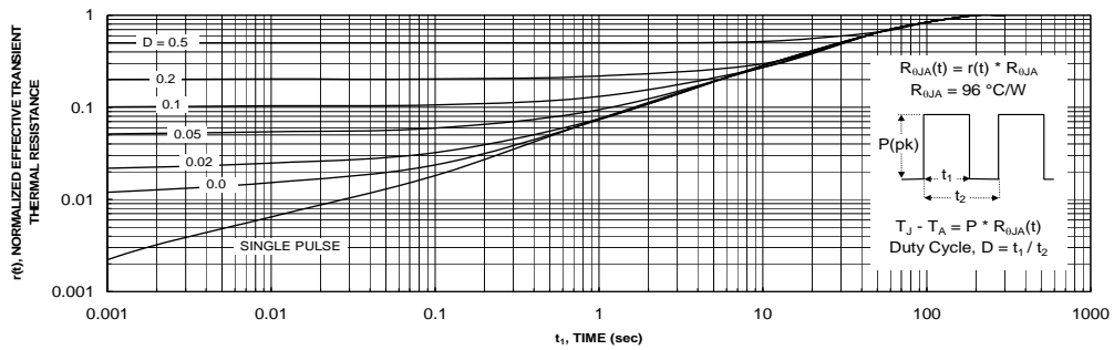
Figure 13. Transient Thermal Response Curve
