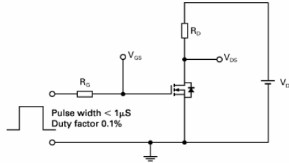
Switching time test circuit
