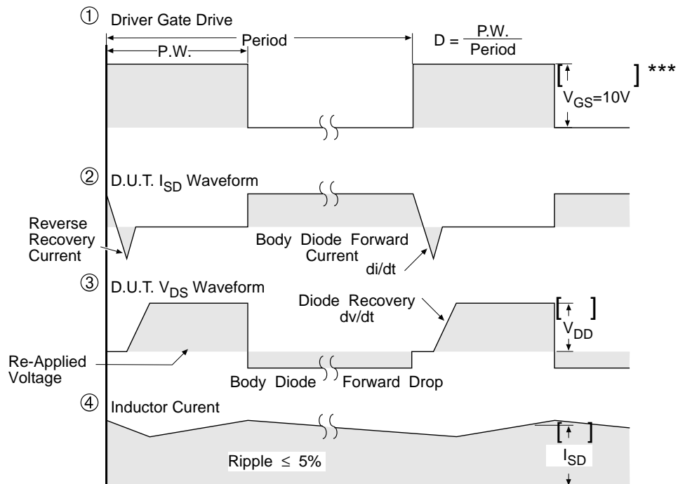
Fig 12. For P-Channel HEXFETS
