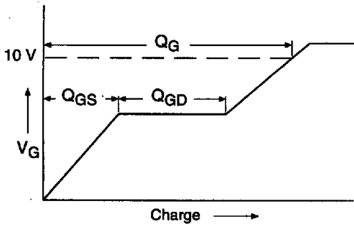
Fig 12a. Basic Gate Charge Waveform
