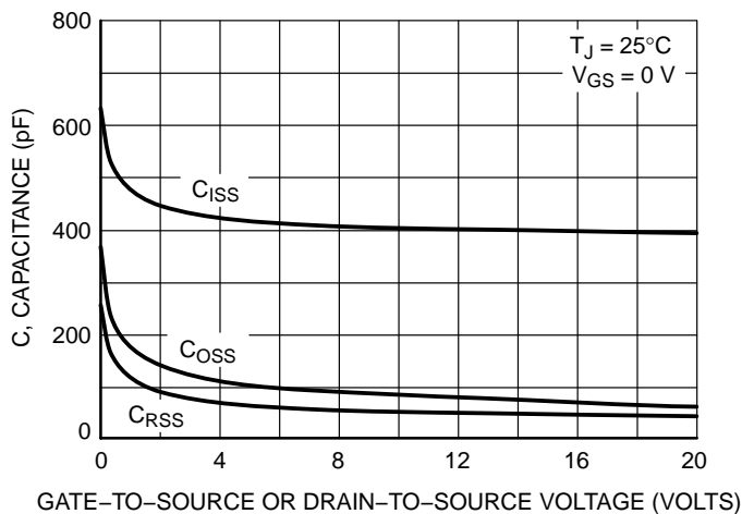
Figure 22. Capacitance Variation
