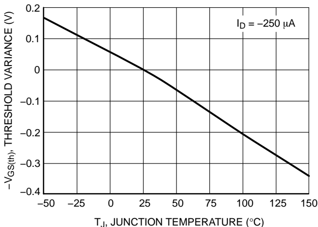
Figure 20. Threshold Voltage
