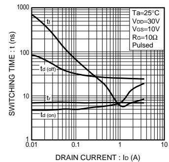
Fig.9 Switching Characteristics
