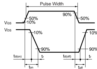
Fig.12 Switching Time Waveforms
