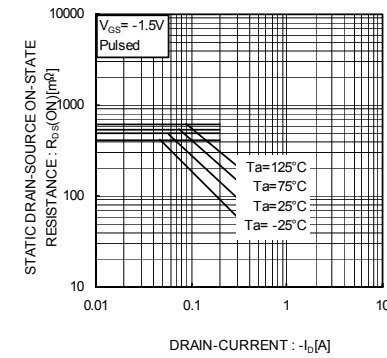
Fig.8 Static Drain-Source On-State Resistance vs. Drain Current (IV)
