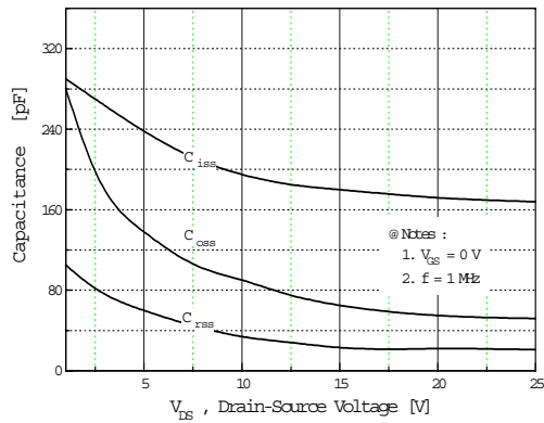
Fig 4. Capacitance vs. Drain-Source Voltage
