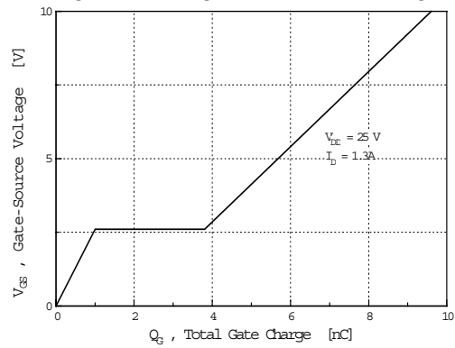
Fig 9. Gate Charge vs. Gate-Source Voltage
