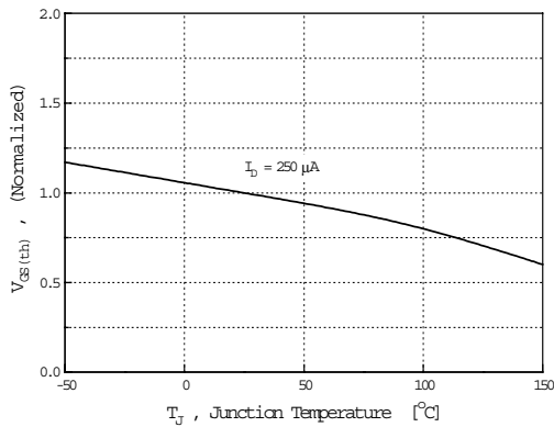
Fig 10. Threshold Voltage
