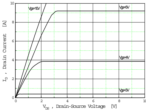
Fig 1. Output Characteristics
