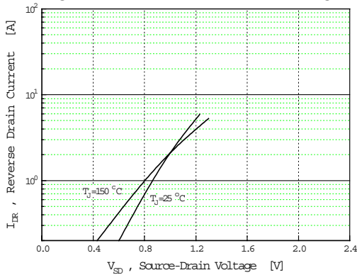
Fig 8. Source-Drain Diode Forward Voltage
