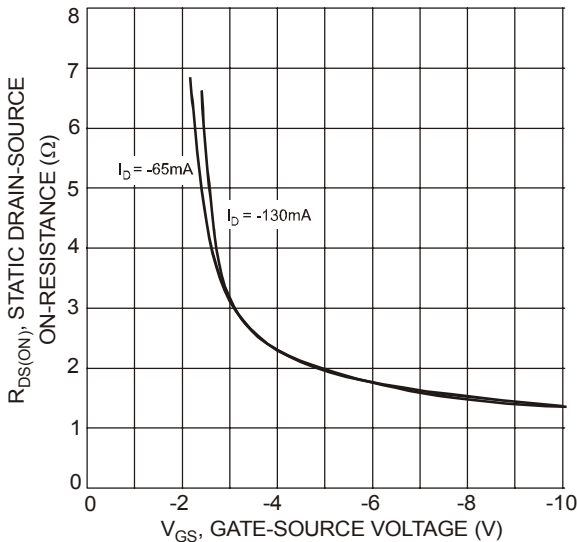
Fig. 5 Static Drain-Source On-Resistance vs. Gate-Source Voltage
