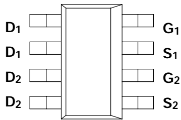
PARTMARKING DETAIL - M4306N
