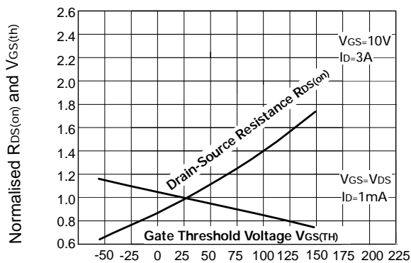
Normalised RDS(on) and VGS(th) v Temperature
