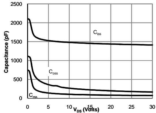
Figure 8: Capacitance Characteristics
