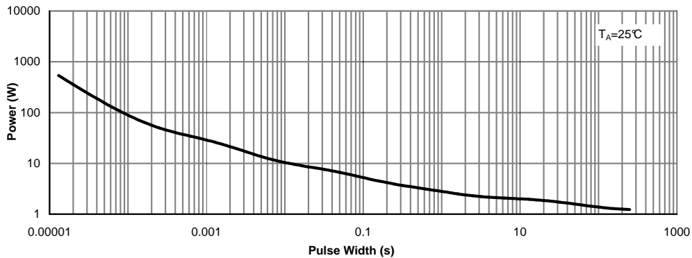
Figure 11: Single Pulse Power Rating Junction-to-Ambient (Note F)
