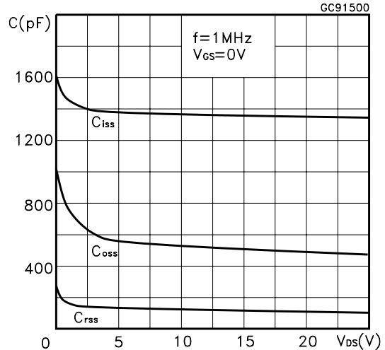
Capacitance Variations
