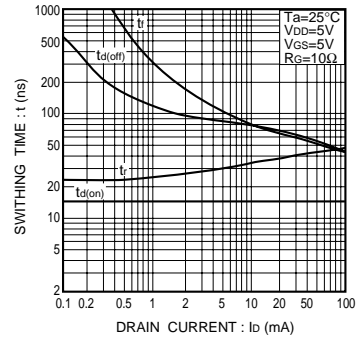
Fig.12 Switching Characteristics
