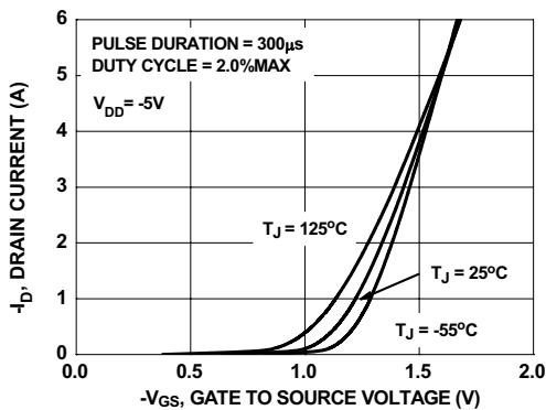
Figure 5. Transfer Characteristics
