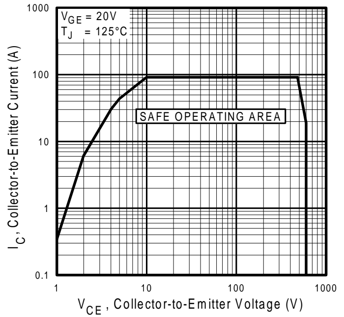
Fig. 12 - Turn-Off SOA
