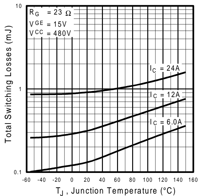
Fig. 10 - Typical Switching Losses vs. Junction Temperature
