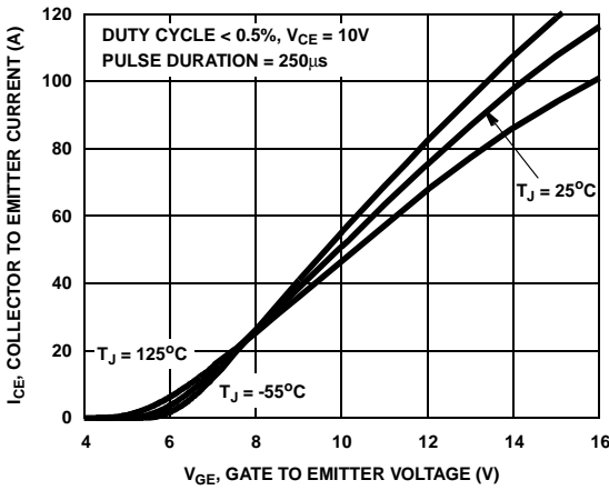
Figure 13. Transfer Characteristic
