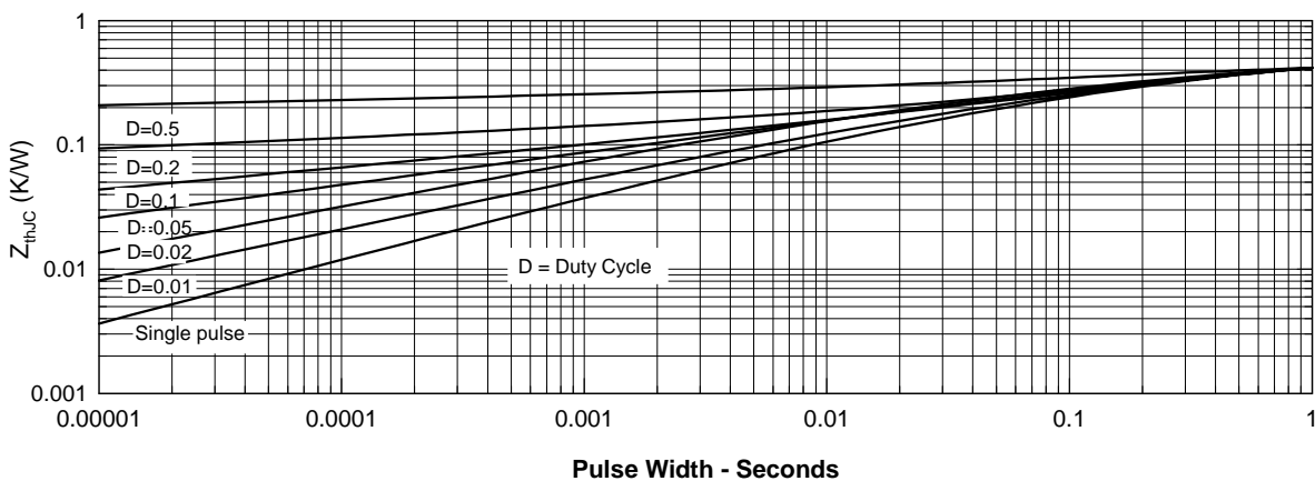
Figure 11. IGBT Transient Thermal Resistance
