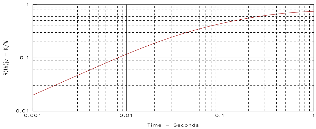
Fig. 18. Diode transient thermal resistance junction-to-case.
