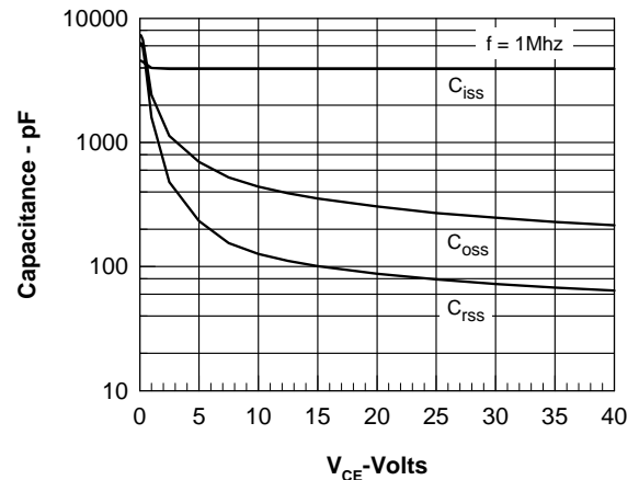
Figure 6. Capacitance Curves
