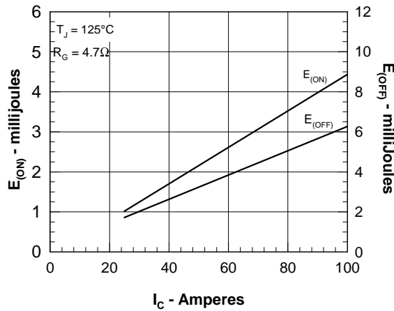
Figure 7. Dependence of E_{ON} and E_{OFF} on I_C .
