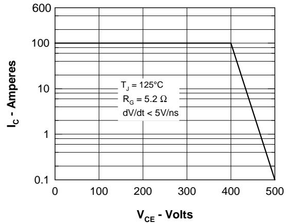
Figure 10. Turn-off Safe Operating Area
