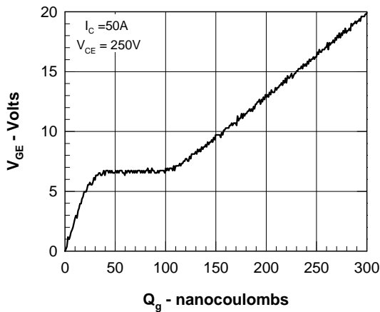
Figure 9. Gate Charge
