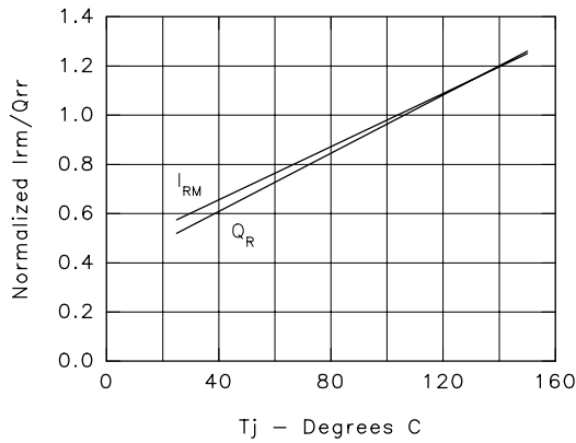
Figure 16. Peak Reverse Recovery Current.
