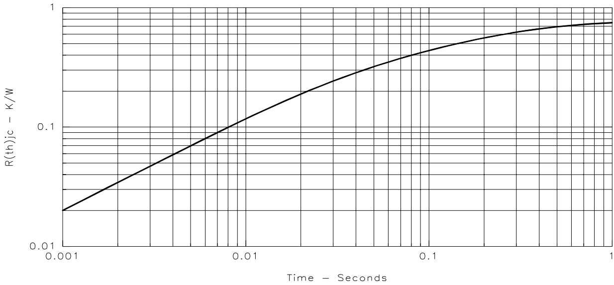
Fig. 18. Diode transient thermal resistance junction-to-case.
