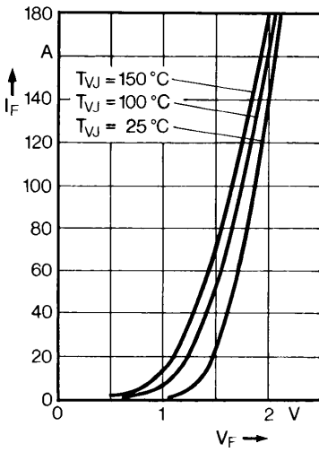
Fig. 12 Forward current versus voltage drop.
