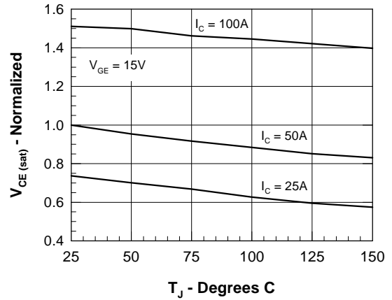
Figure 4. Temperature Dependence of V_{CE(sat)}
