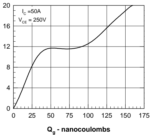
Figure 9. Gate Charge
