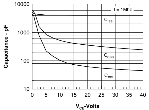
Figure 6. Capacitance Curves
