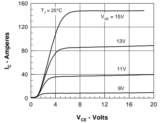
Figure 2. Extended Output Characteristics
