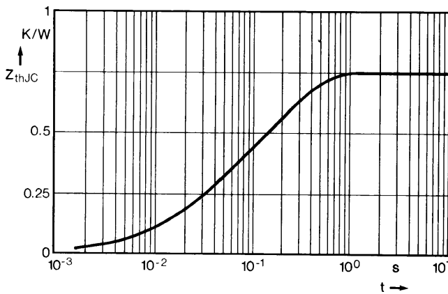
Fig. 18 Transient thermal impedance junction to case.
