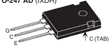
G = Gate, E = Emitter C = Collector, TAB = Collector
