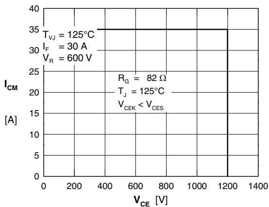
Fig. 9 Reverse biased safe operating area RBSOA
