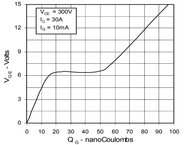
Fig. 14. Gate Charge
